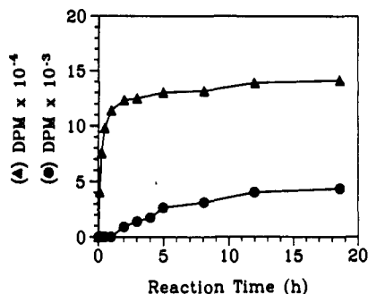
Figure 1. Progress curve for synthesis of ( S )-12-OP ( \blacktriangle ) and ( S )-14-OP ( \bullet ) by cell-free extracts from M. thermoautotrophicum . Incubation of ( S )-[1- 3 H]3-OP and 5-OPP was at 37 °C. Samples were hydrolyzed with alkaline phosphatase, and ether extracts were analyzed by reversed-phase HPLC.
